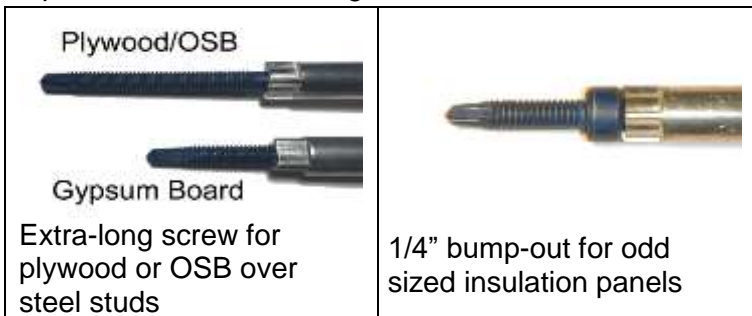
Steel Stud backup – Pos-I-Tie® Barrel Screw penetrates gypsum sheathing and insulation
