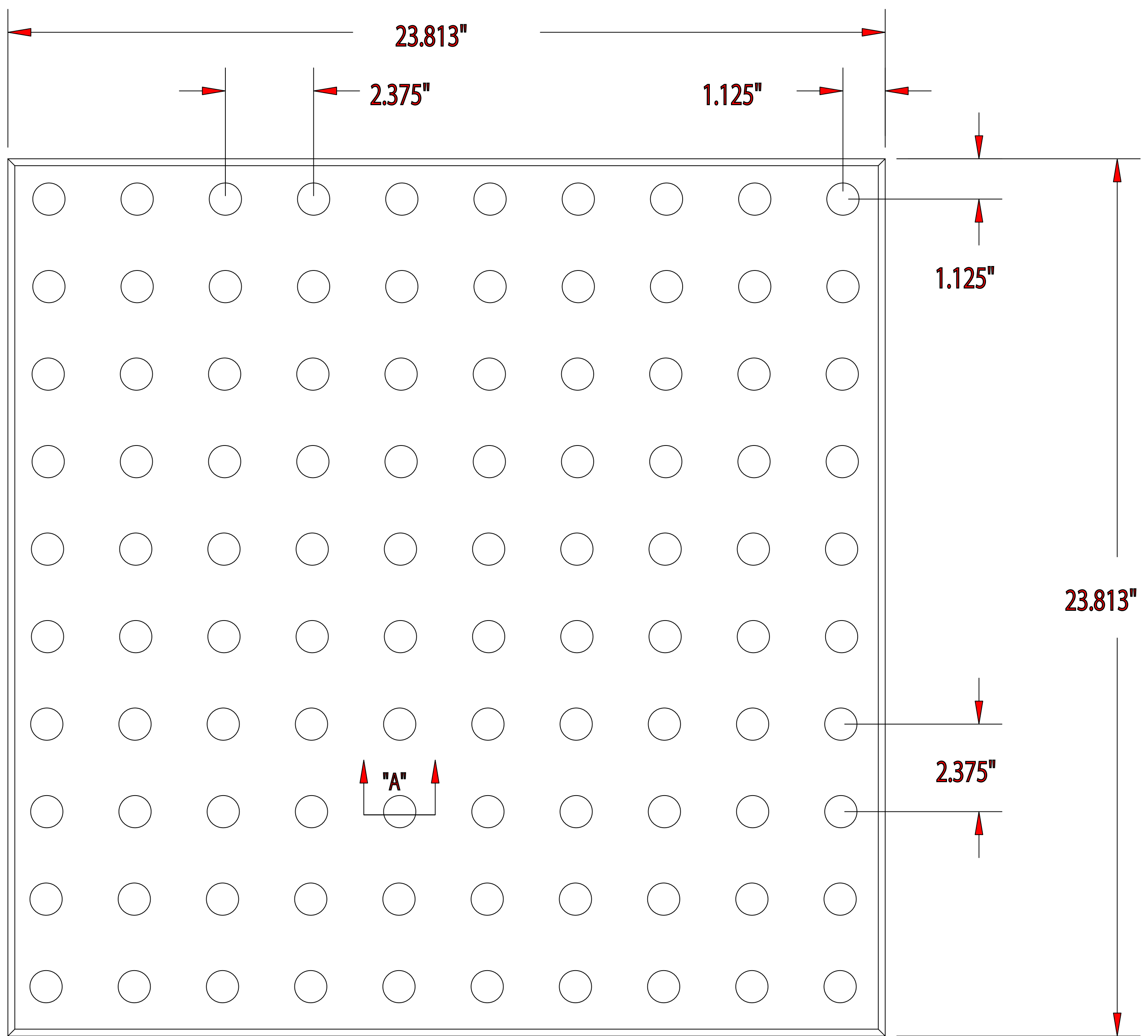
24" ADA-2 PAVER
