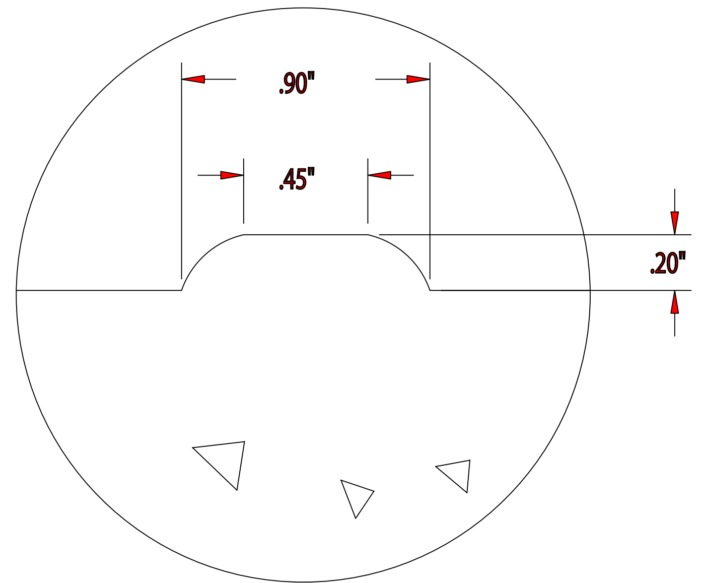
DETAIL 'A' WARNING DOME DETAIL
