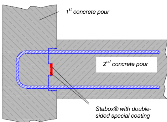
System Diagram
