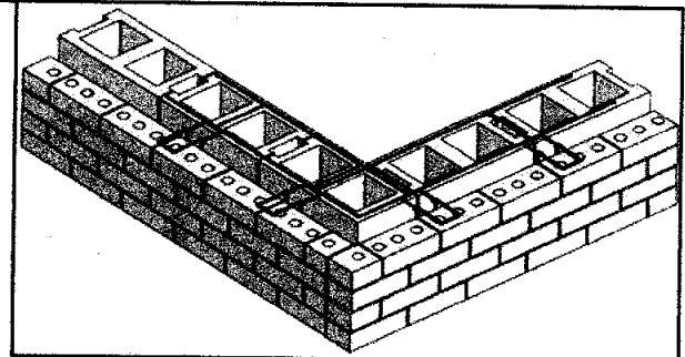
PREFABRICATED CORNER
