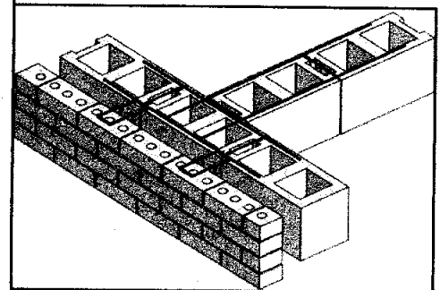
PREFABRICATED TEE
