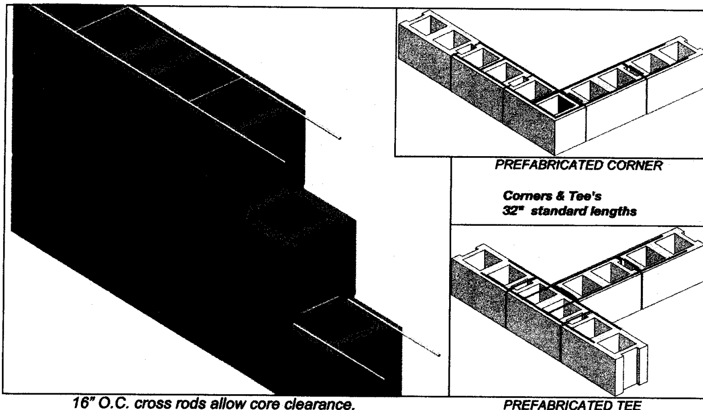
PREFABRICATED TEE
